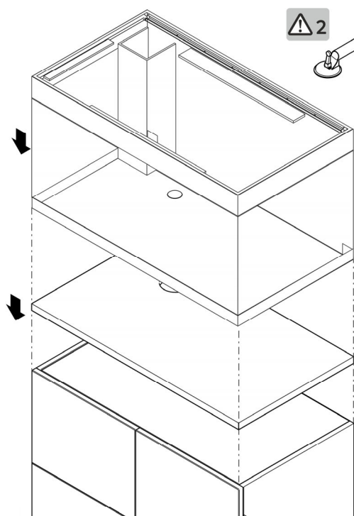
HighLine 125, 175, 200, 300, 400, 600
