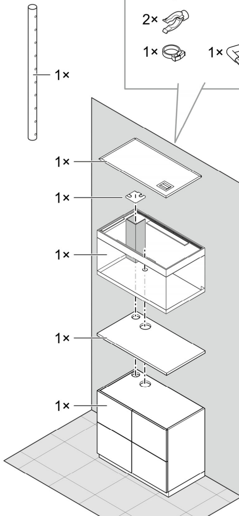
HighLine 125, 175, 200, 300, 400, 600
