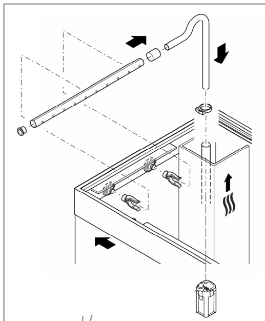
HighLine 125, 175, 200, 300, 400, 600
